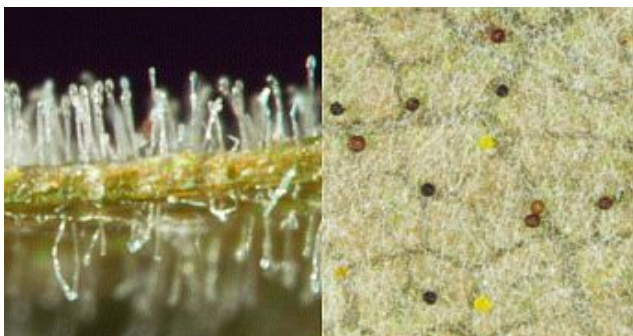
Figure 3. Left: Cross-section of a grape leaf covered in powdery mildew with new conidia developing at the end of the stalks. Right: Immature (yellow) and mature (black) cleistothece on a Sultana leaf in early autumn.
